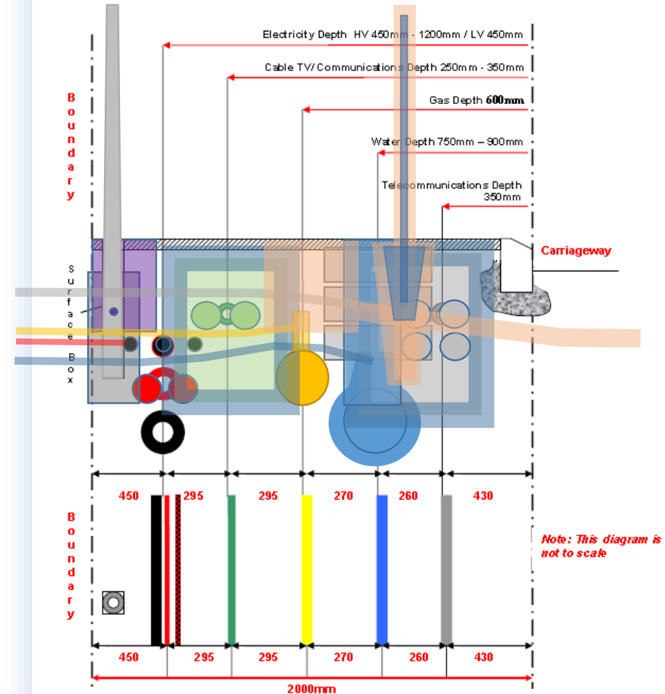
FIGURE 1 - Recommended Positioning of Utility Apparatus in a 2 metre Footway
